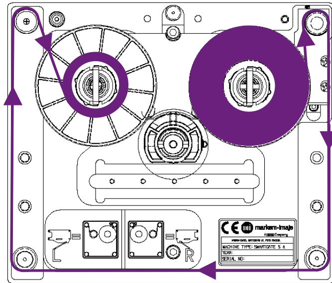
SmartDate X60 LH Cassette Ribbon Web Path
